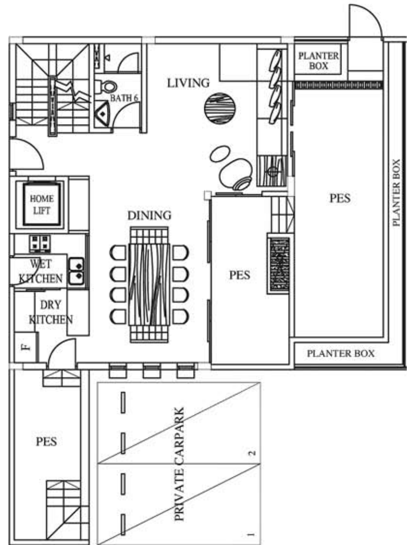
1ST STOREY PLAN
