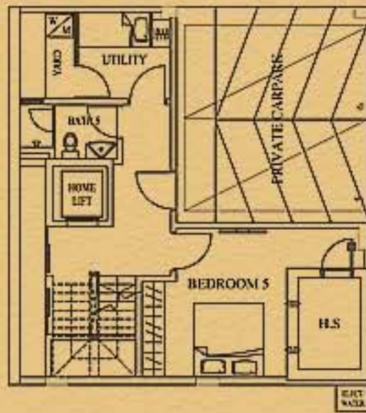
BASEMENT PLAN
